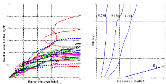
Fig 2 Figure 2. IDA results for the reference frame: (a) twenty IDA curves and their median, (b) median interstorey drift demands for different, S a(T^*, 5\%) values
